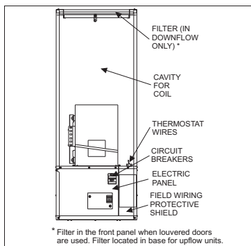
FIGURE 1: Component Locations
